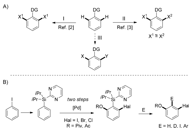
Scheme 1. Twofold C–H functionalization adjacent to a directing group (DG). A) I, II) Previously reported bisfunctionalization with two identical or similar groups; III) unsymmetrical bisfunctionalization. B) The approach developed in this study for unsymmetrical bisfunctionalization.
